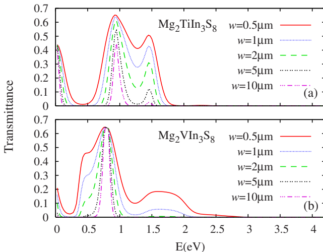
FIG. 12. (Color online) Transmittance of the intermediate-band derivatives of MgIn 2 S 4 as a function of the width of the sample w .
