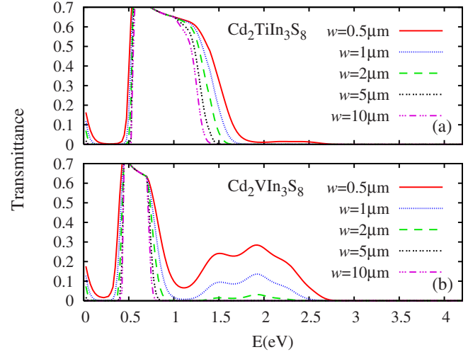
FIG. 13. (Color online) The same as Fig. 12, but for the derivatives of CdIn 2 S 4 .
